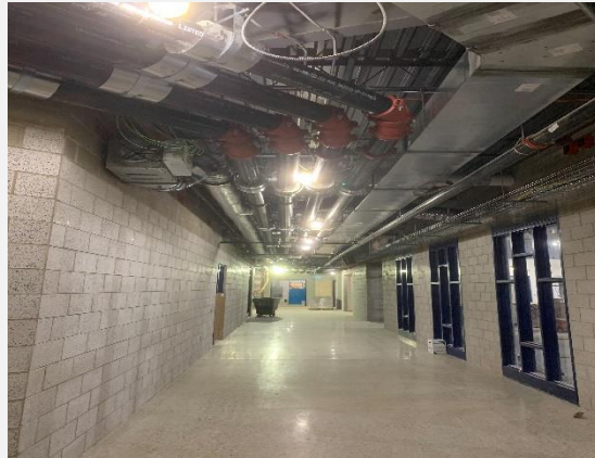
New Piping, Ductwork, & Electrical
