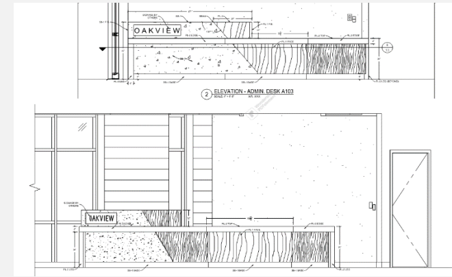
Oakview - New Reception Desk Shop Drawing
