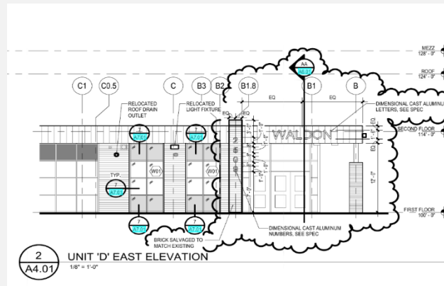
Waldon - New Elevation of Added Windows
