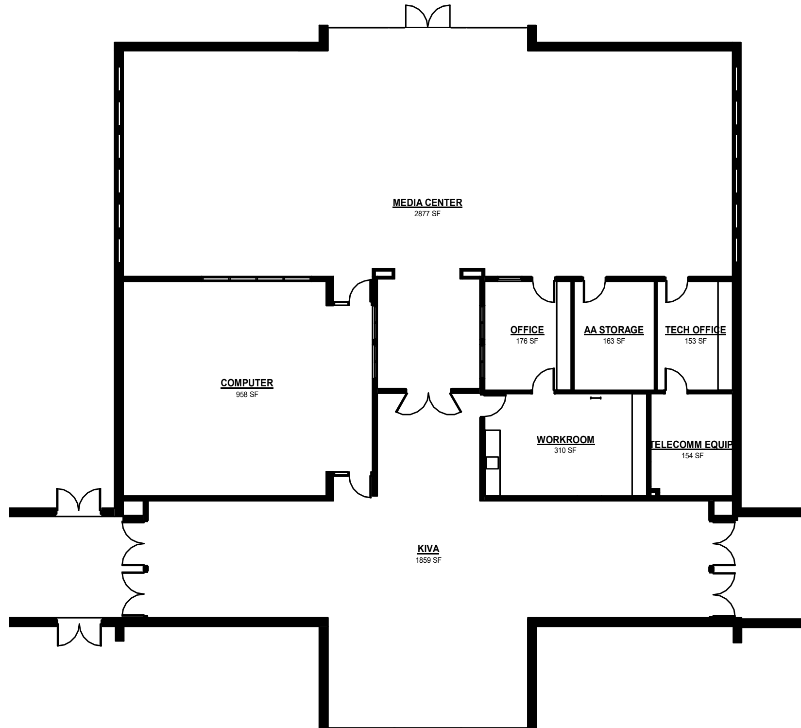
ENLARGED EXISTING FLOOR PLAN
